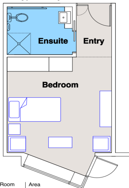
Typical Layout 1:50
